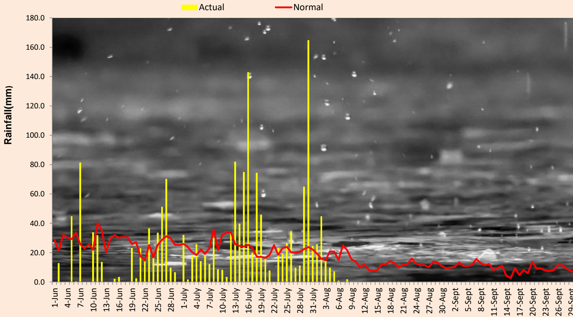
Daily Average Rainfall for CWRDM (Kozhikode)-SW Monsoon 2024
