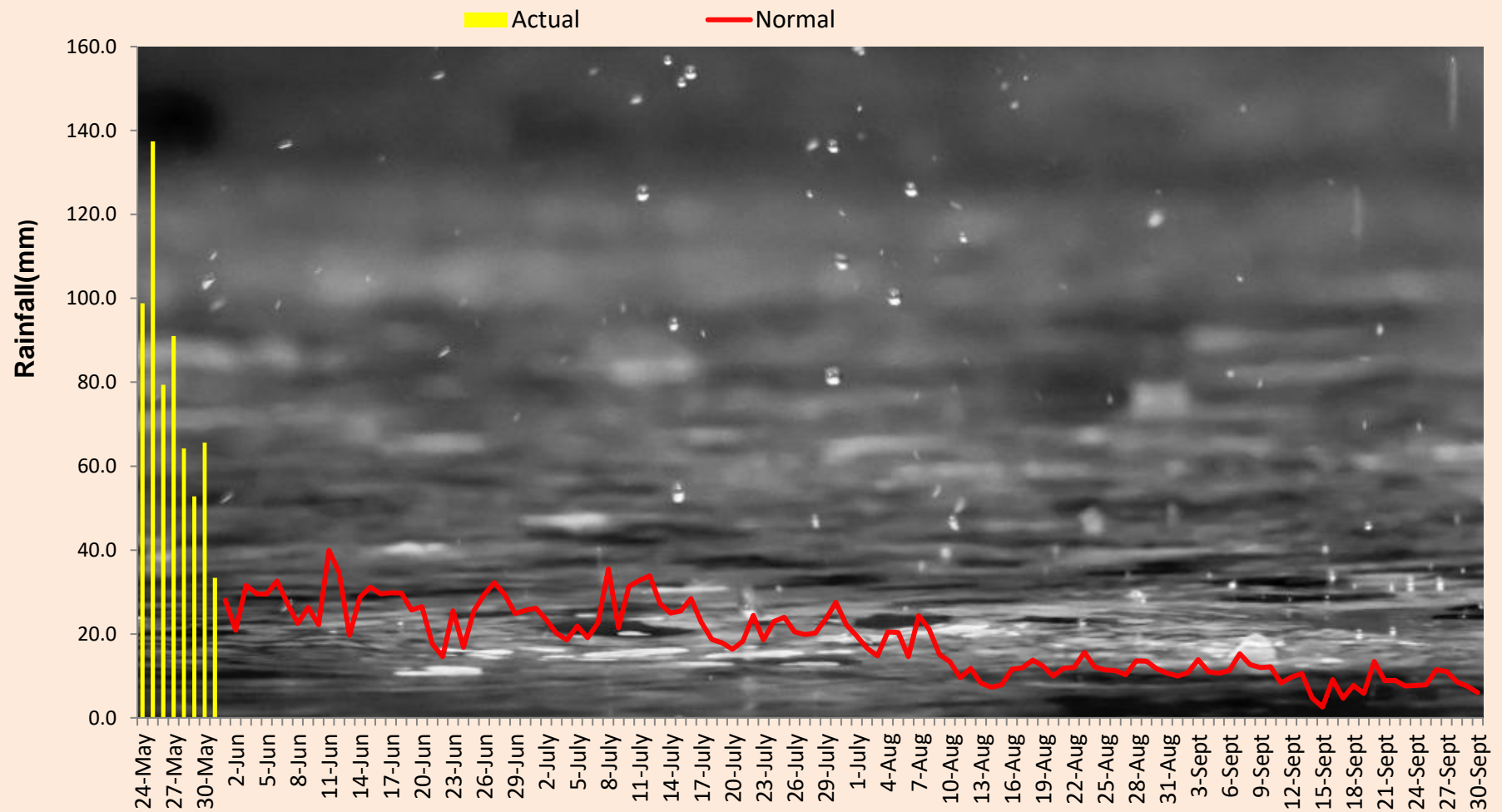
Daily Average Rainfall for CWRDM (Kozhikode)-SW Monsoon 2025
