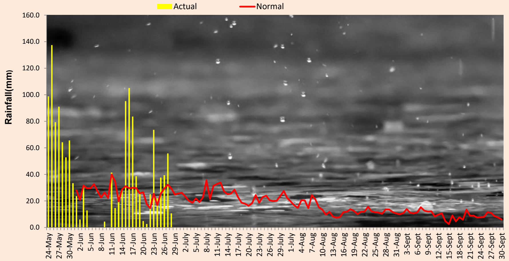
Daily Average Rainfall for CWRDM (Kozhikode)-SW Monsoon 2025
